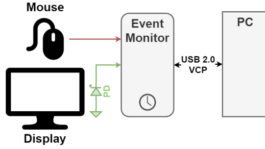
Figure 2: Mouse to photon logger configuration
