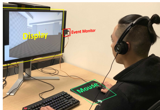
Figure 1: The hardware setup used including the mouse, display, desktop PC and Click-to-Photon logger (Section 2).
